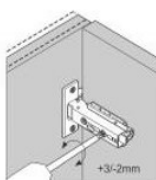
Depth adjustment via worm gear
