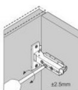
Height adjustment via base plate
